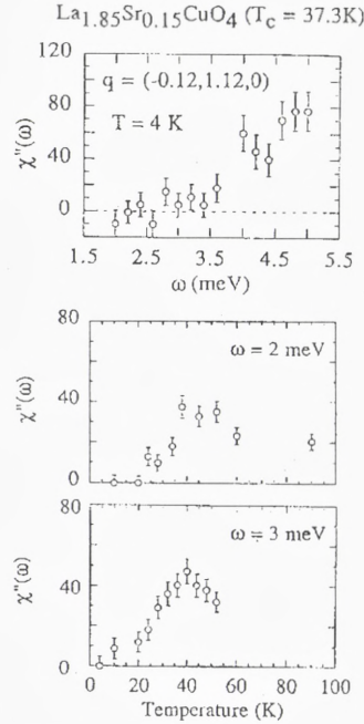
Figure 4. \chi''(q = Q_\delta, \omega) is plotted as the function of transfer energy, \omega at T = 4\text{ K} (top). Temperature dependence for \omega = 2\text{ meV} (middle), and 3\text{ meV} (bottom) are also shown (Yamada et al., 1995).
