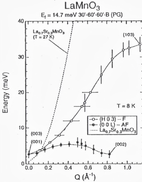
Figure 6. Spin-wave dispersion curves of \text{LaMnO}_3 along (100) and (001) directions (orthorhombic notation). The isotropic ferromagnetic spin-wave dispersion of \text{La}_{0.7}\text{Sr}_{0.3}\text{MnO}_3 is shown as the reference (Hirota et al., 1996).
